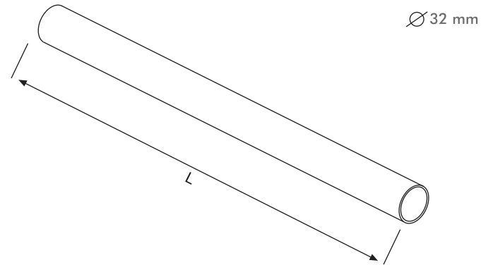
Bumper Suitable For Base Leg Reyon Önü Bariyer Borusu
