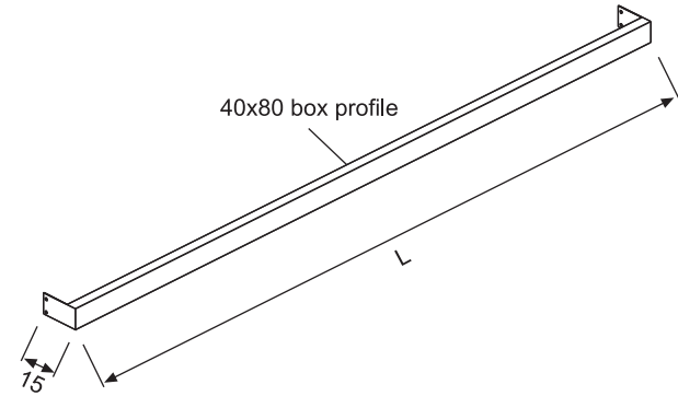
Safety Crossbeam Dayama Traversi
