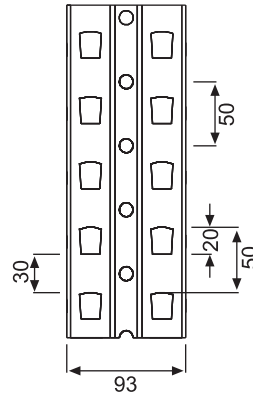
Frame Detail Ayak Kesiti
